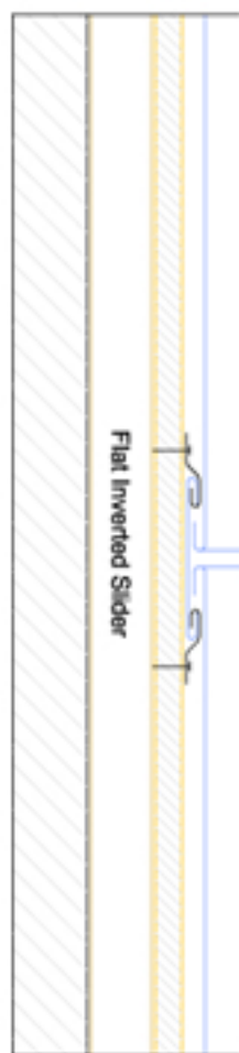
Transversal junction 90°
