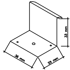
Zinc sheet clip
