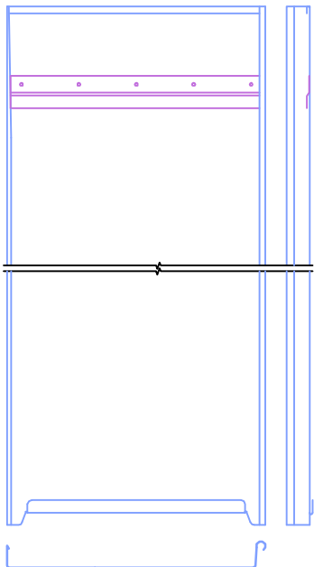
PANEL DETAILS 1:10
