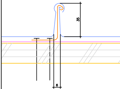
PANEL DETAILS 1:10
