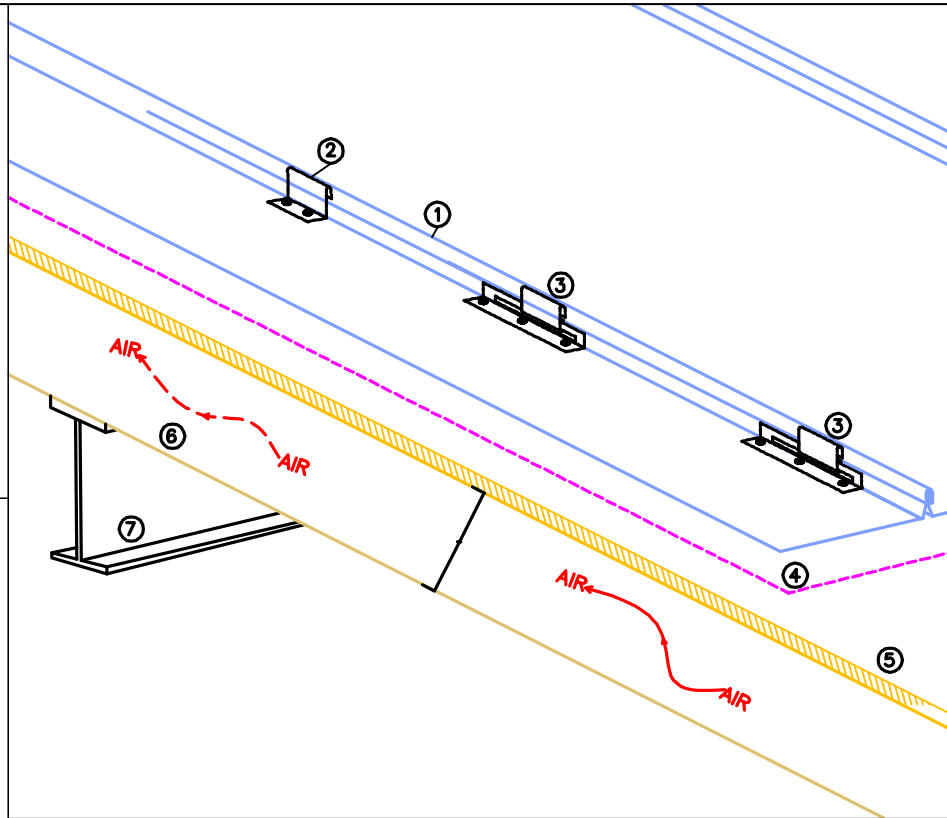
fixed clip
