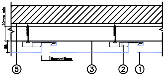
GROOVED JOINT
