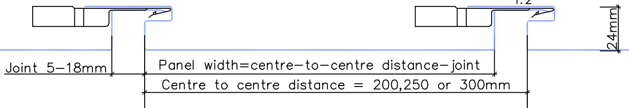
PANEL SECTION 1:2
