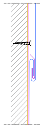
TRANSVERSAL JOINT 1:2
