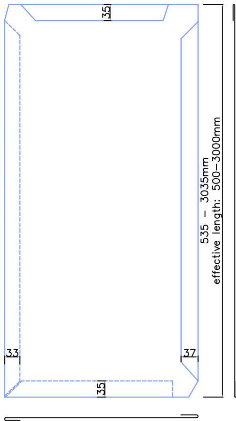
PANEL DETAIL 1:8
