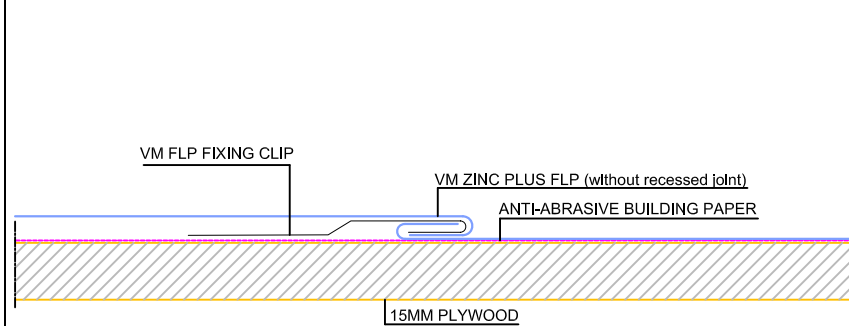
LAYING FRAMEWORK
