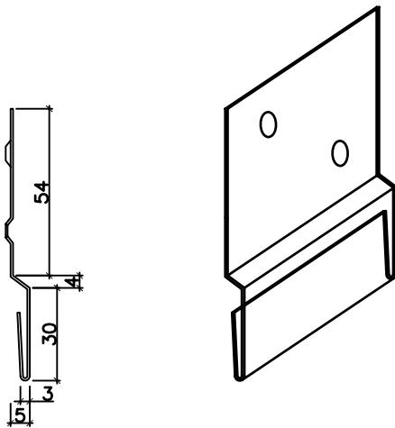
PANEL DETAIL 1:8
