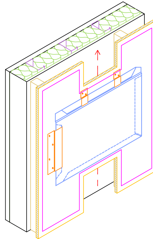
LAYING FRAMEWORK
